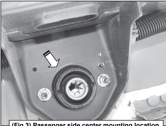
(Fig 3) Passenger side center mounting location
